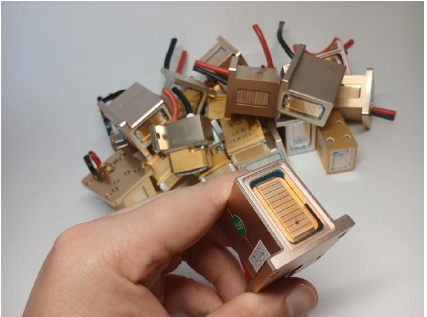
Diode assembly for a laser handle
